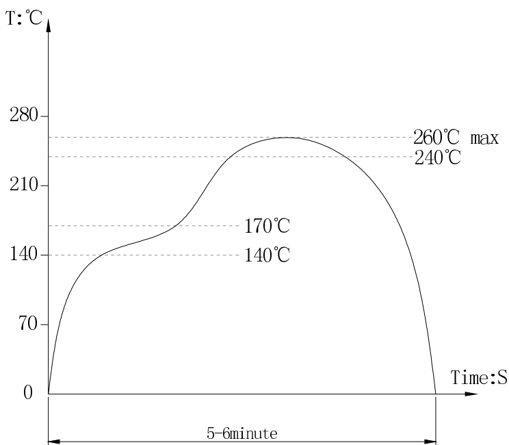
< Temperature profile >
